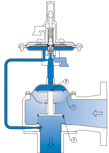
Open Condition—Direct Actuated
